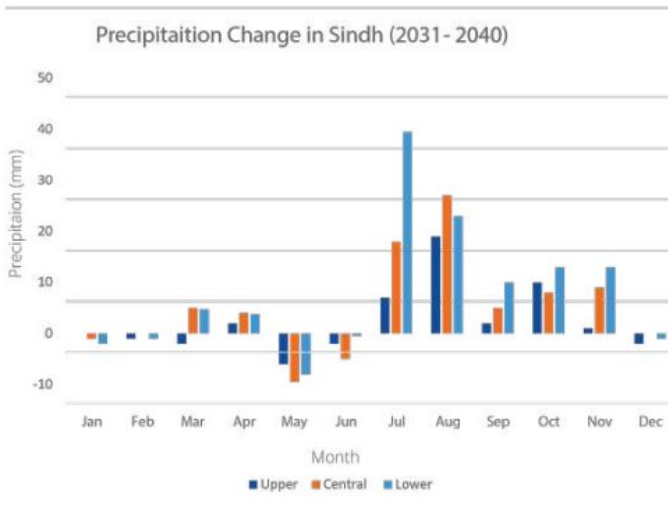
Future projections of precipitation for lower, central and upper parts of the Sindh 5
