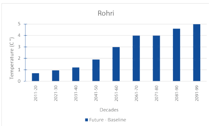
Mean daily future temperature projections for the Indus Delta on decadal basis during 21st century 6
