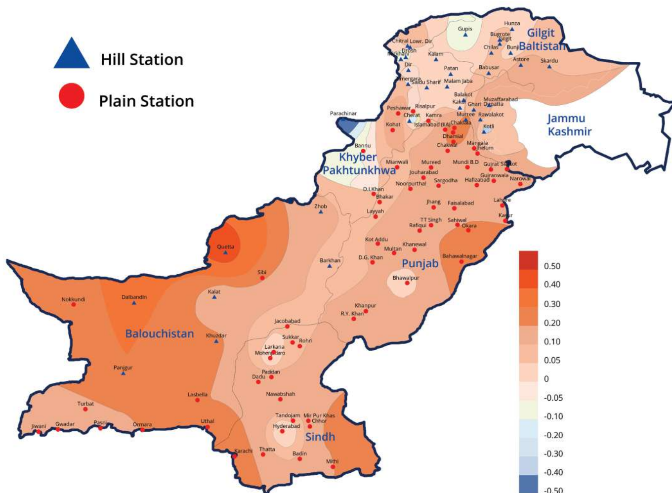
Spatial distribution of mean annual temperature trends, 1961 to 2018 ( ^{\circ}\text{C}/\text{decade} ) 4
